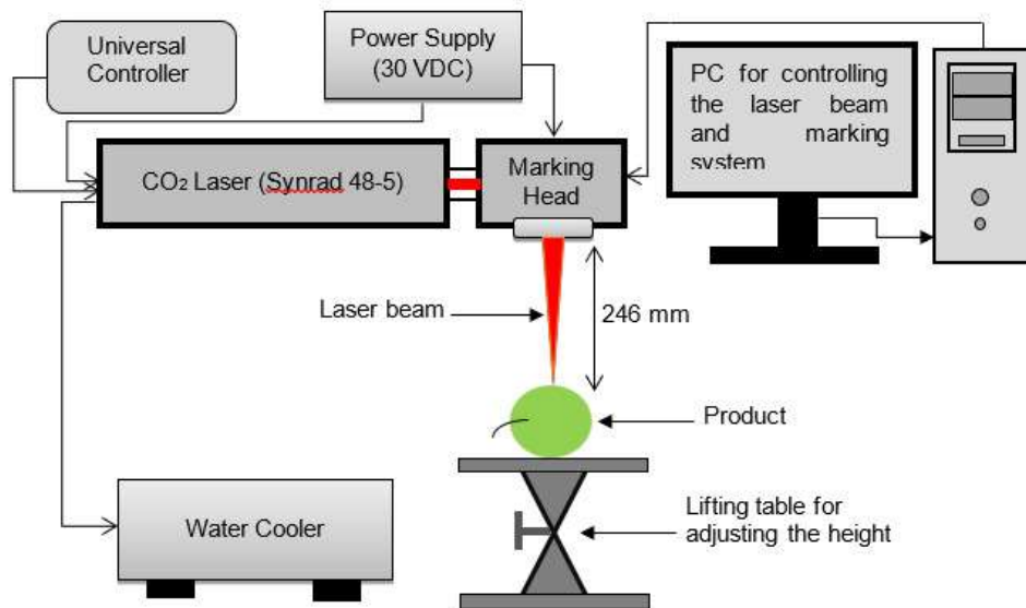
Figure 1. Laser marking experiment setup showing the CO 2 laser. CO 2 Laser: Synrad 48-5 (manufacturer: Synrad, model: 48-5), Power Supply: 30 VDC unit for laser operation. Marking Head: Not enough detail is provided in the image. For clarity, authors should include the manufacturer and model of the marking head in the manuscript. PC Controller: Used for software-based control of laser marking parameters. Universal Controller & Water Cooler: Supportive systems for laser operation and cooling. Product Positioning System: Lifting table, which requires manual height adjustment to position the product correctly.
