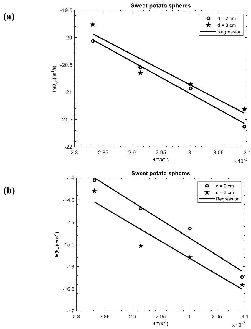
Figure S1. Representation by the Arrhenius-type equation for drying spherical sweet potatoes: (a) of moisture diffusivity; (b) convective mass transfer coefficient.
