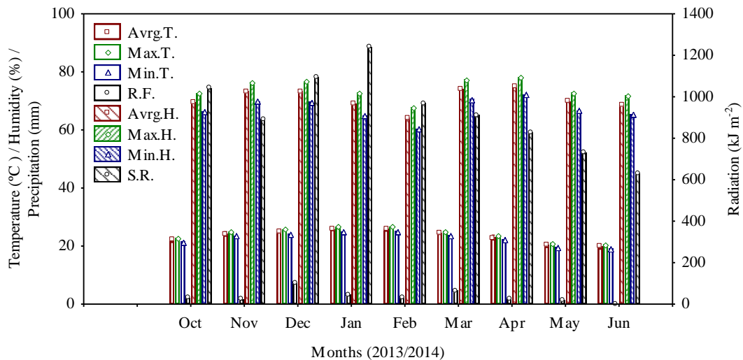
Fig 7. Climate diagrams variables recorded during the experimental period, average (Avg.T.), maximum (Max.T.), and minimum temperatures (Min.T.), rainfall (R.F.), average (Avg.H.), maximum (Max.H.), and minimum (Min.H.) relative humidity and solar radiation (S.R.).
